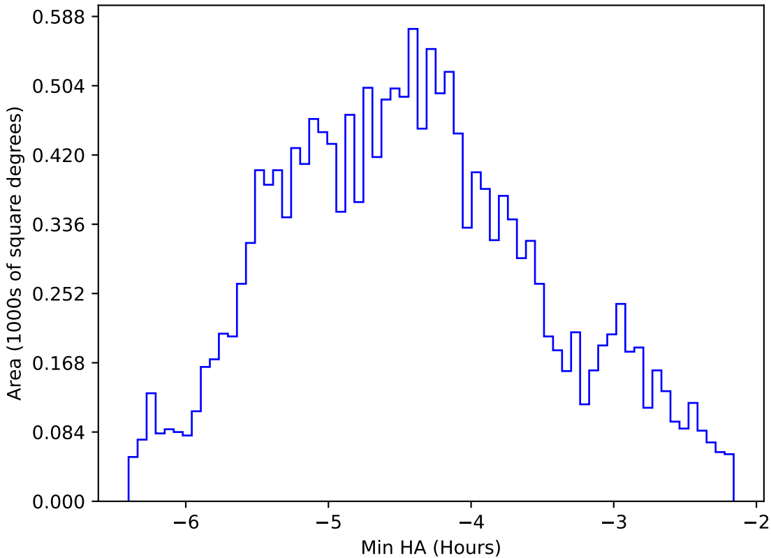
too_ignore_100_1v3.4_10yrs WFD r band: Min HA
