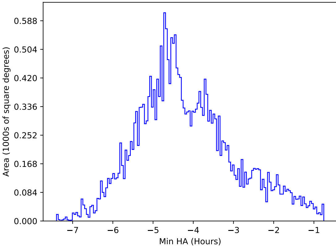
too_ignore_100_1v3.4_10yrs All sky z band: Min HA
