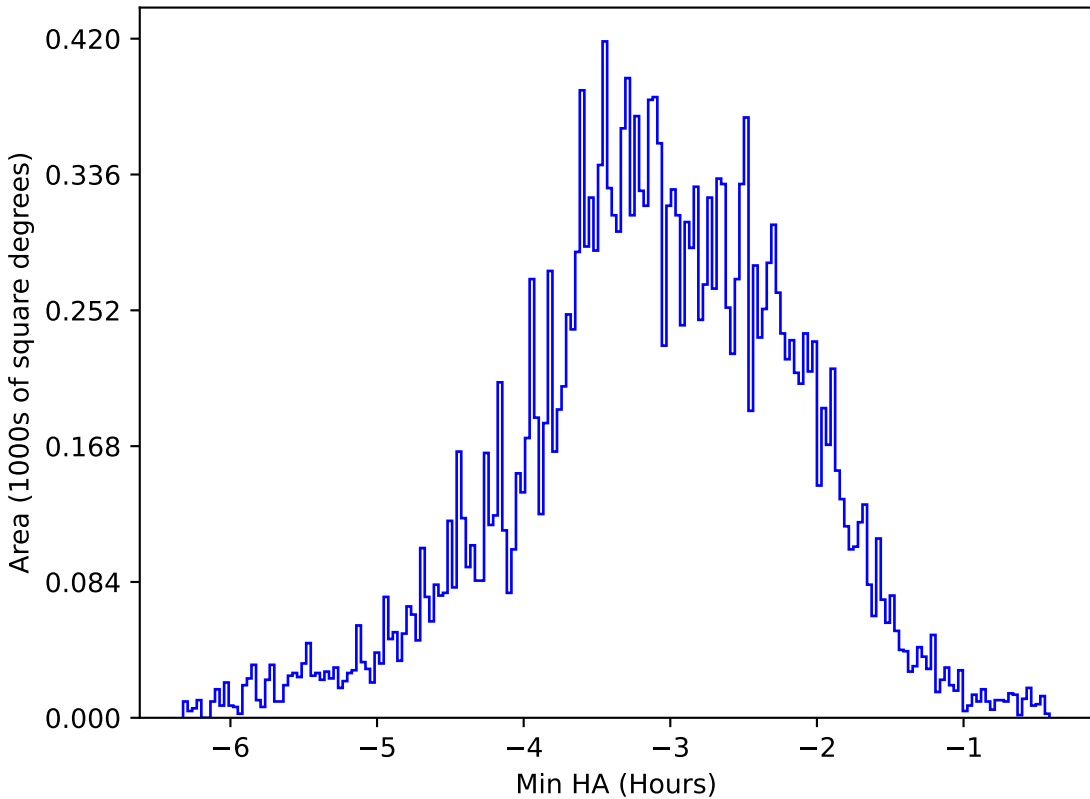
too_ignore_100_1v3.4_10yrs All sky u band: Min HA
