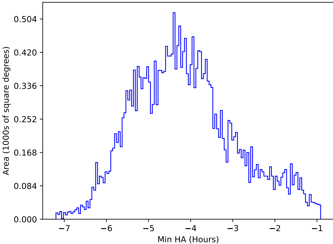
too_ignore_100_1v3.4_10yrs All sky r band: Min HA
