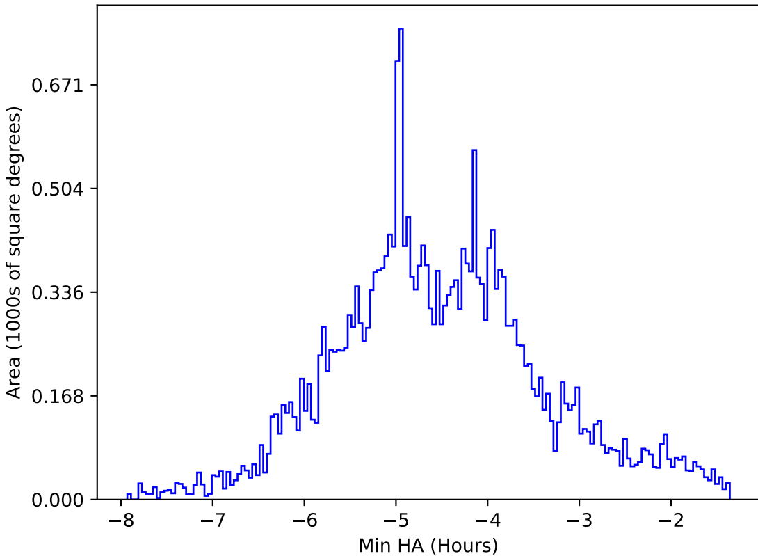
too_ignore_100_1v3.4_10yrs All sky all bands: Min HA
