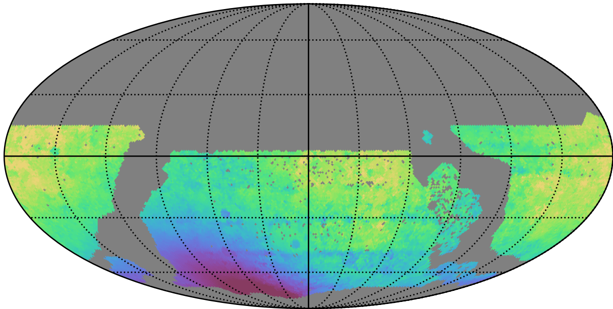
too_ignore_100_1v3.4_10yrs WFD z band: Median solarElong
