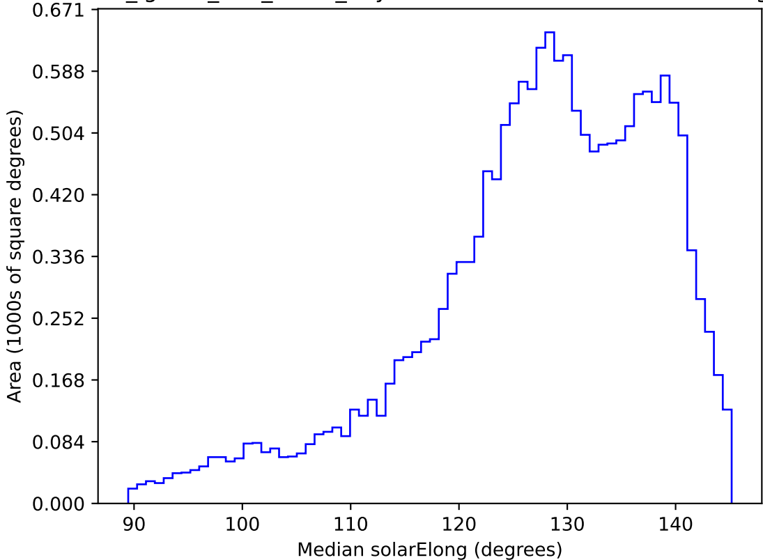
too_ignore_100_1v3.4_10yrs WFD z band: Median solarElong
