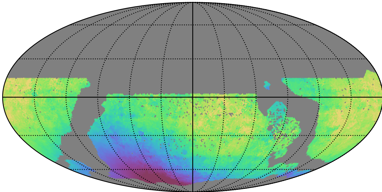
too_ignore_100_1v3.4_10yrs WFD y band: Median solarElong
