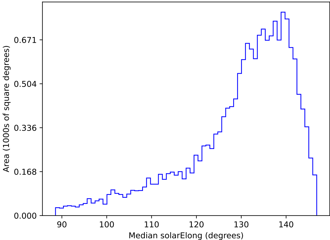
too_ignore_100_1v3.4_10yrs WFD y band: Median solarElong
