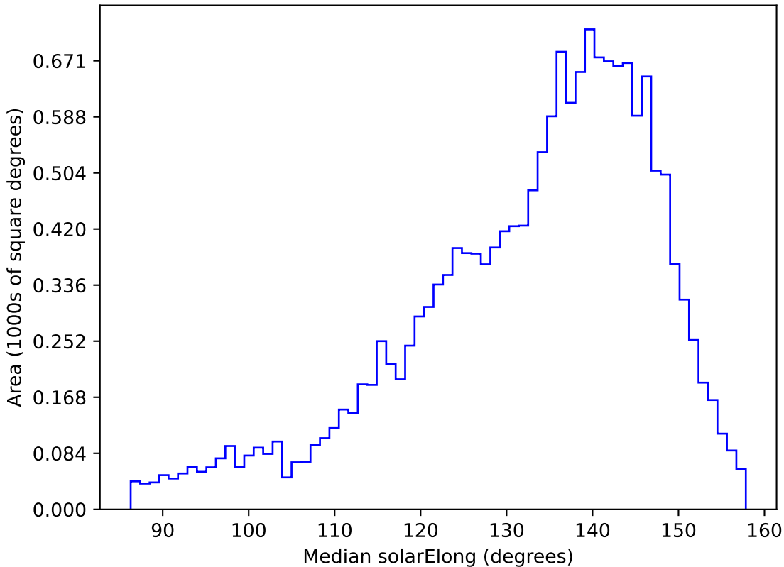
too_ignore_100_1v3.4_10yrs WFD u band: Median solarElong
