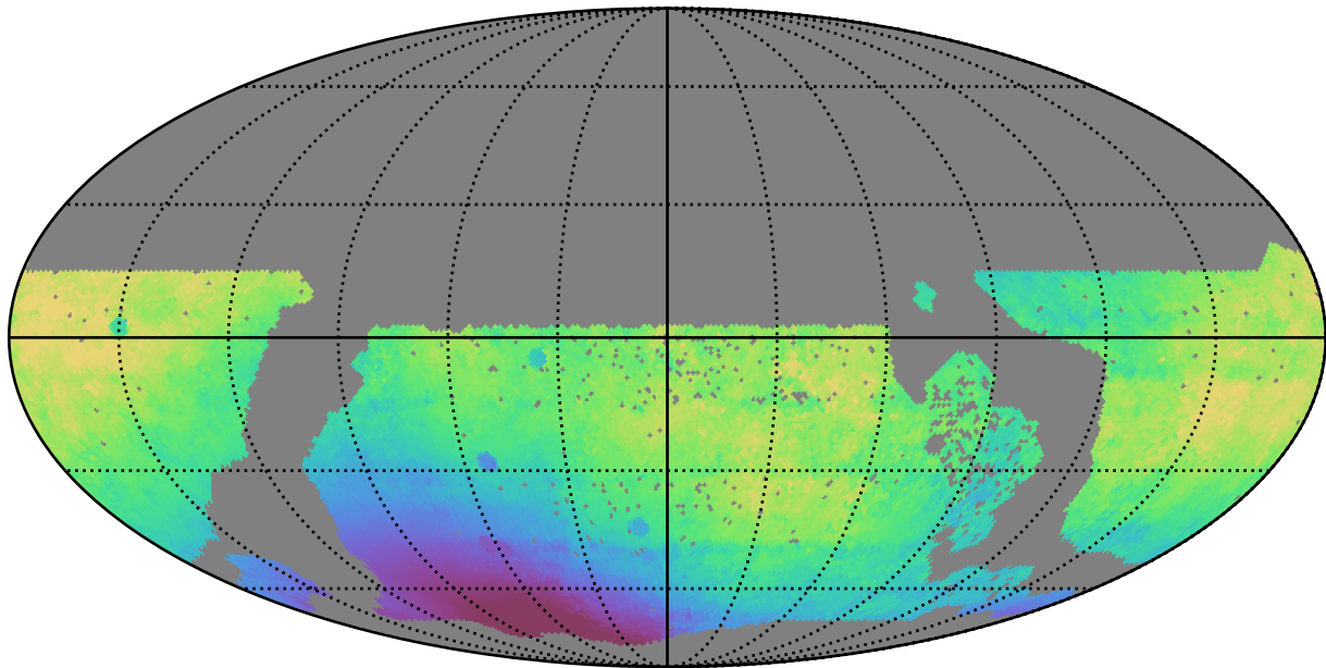
too_ignore_100_1v3.4_10yrs WFD r band: Median solarElong
