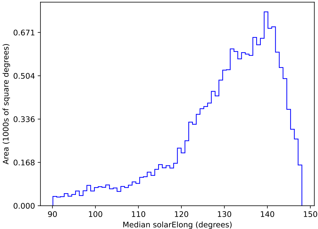
too_ignore_100_1v3.4_10yrs WFD r band: Median solarElong
