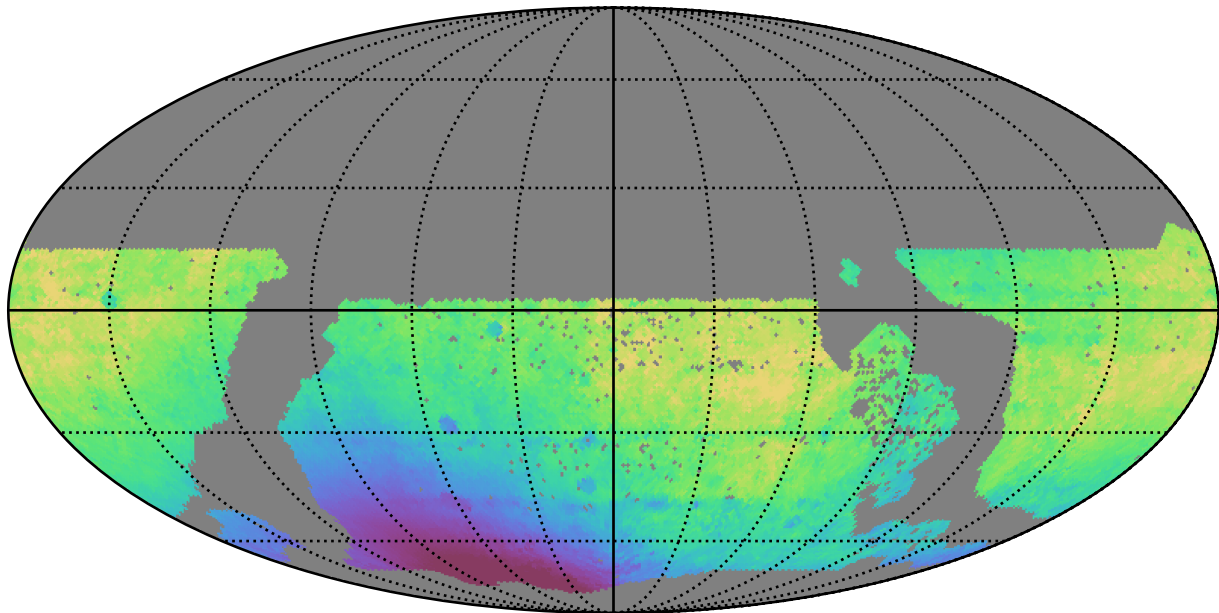
too_ignore_100_1v3.4_10yrs WFD i band: Median solarElong
