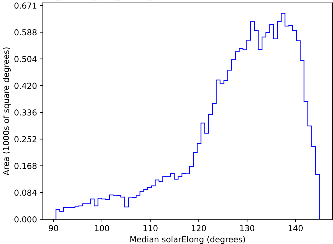
too_ignore_100_1v3.4_10yrs WFD i band: Median solarElong
