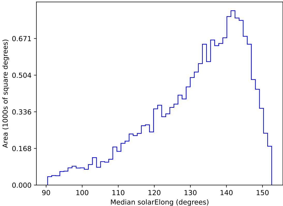
too_ignore_100_1v3.4_10yrs WFD g band: Median solarElong
