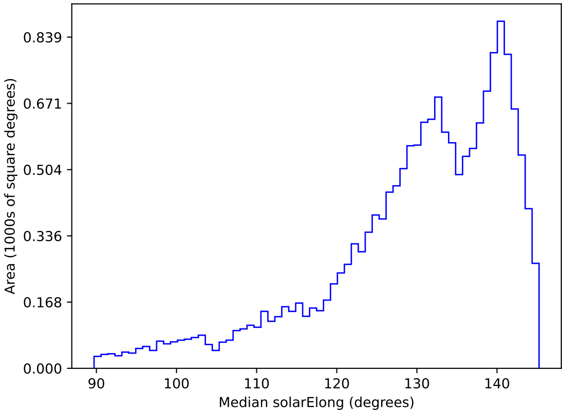
too_ignore_100_1v3.4_10yrs WFD all bands: Median solarElong
