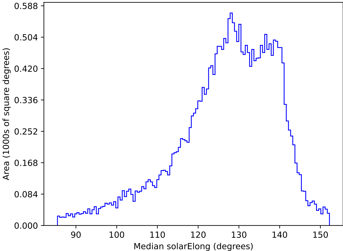
too_ignore_100_1v3.4_10yrs All sky z band: Median solarElong
