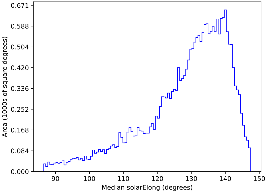
too_ignore_100_1v3.4_10yrs All sky y band: Median solarElong
