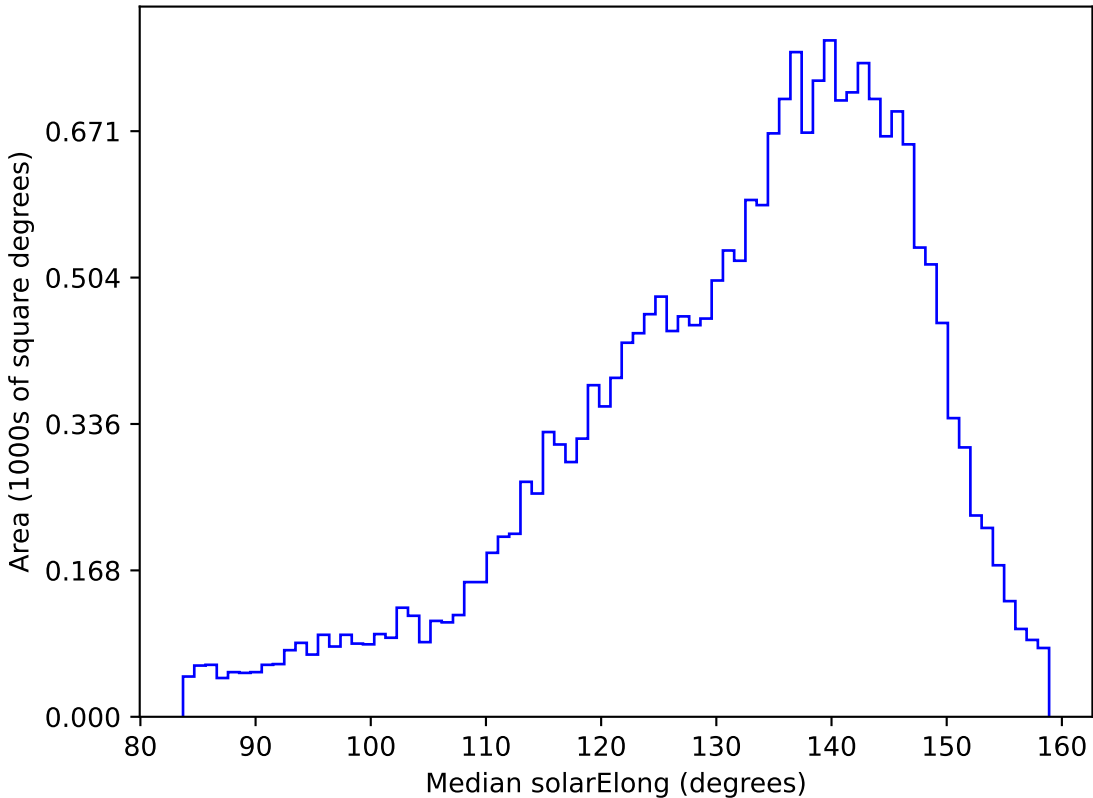
too_ignore_100_1v3.4_10yrs All sky u band: Median solarElong
