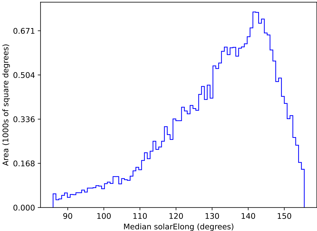
too_ignore_100_1v3.4_10yrs All sky g band: Median solarElong
