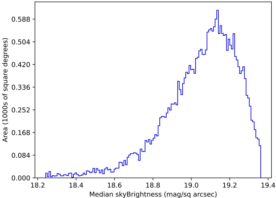
too_ignore_100_1v3.4_10yrs Yr 1 z band: Median skyBrightness
