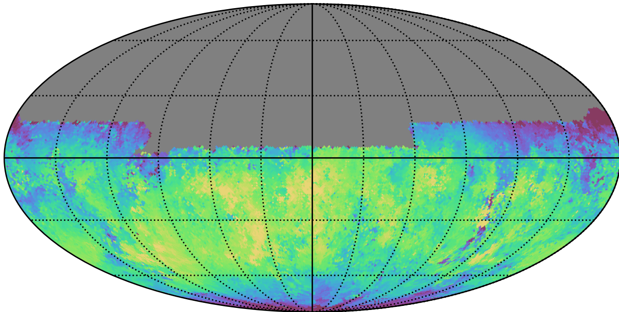
too_ignore_100_1v3.4_10yrs Yr 1 y band: Median skyBrightness
