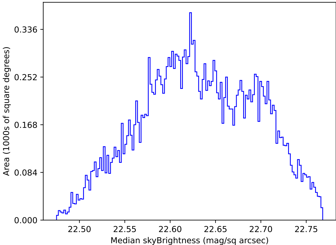
too_ignore_100_1v3.4_10yrs Yr 1 u band: Median skyBrightness
