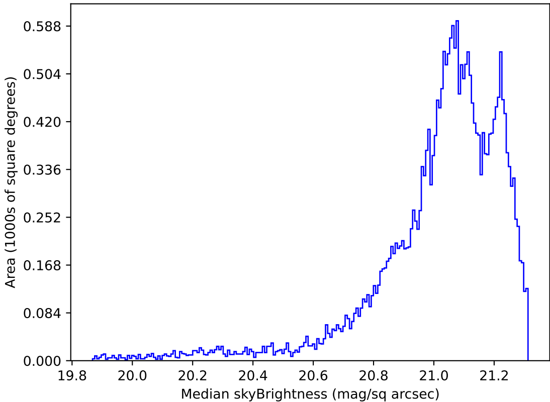
too_ignore_100_1v3.4_10yrs Yr 1 r band: Median skyBrightness
