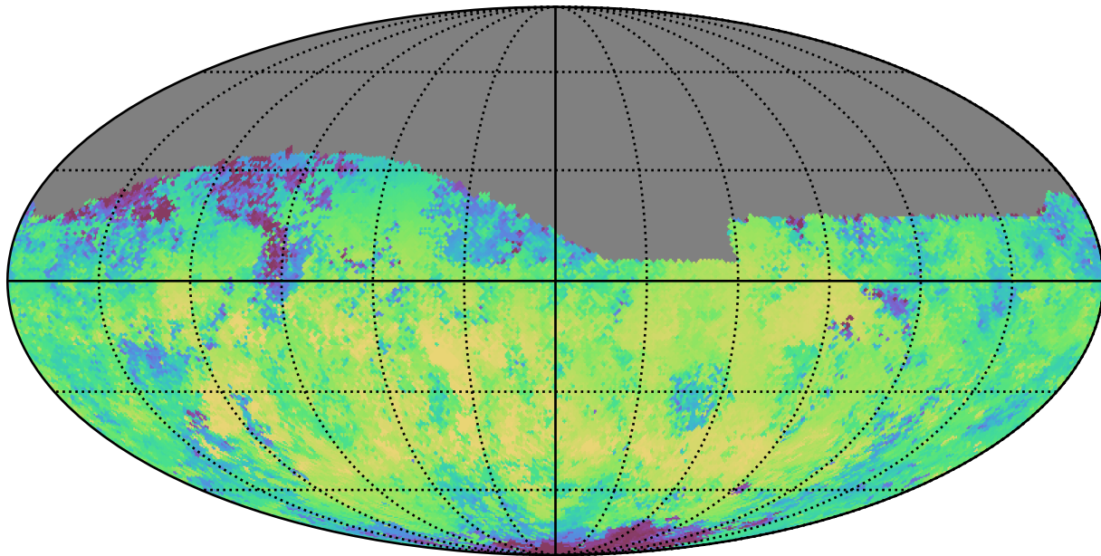
too_ignore_100_1v3.4_10yrs Yr 1 i band: Median skyBrightness
