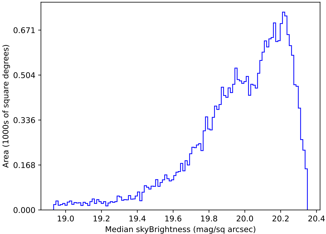
too_ignore_100_1v3.4_10yrs Yr 1 i band: Median skyBrightness
