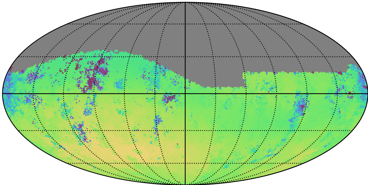
too_ignore_100_1v3.4_10yrs Yr 1 g band: Median skyBrightness
