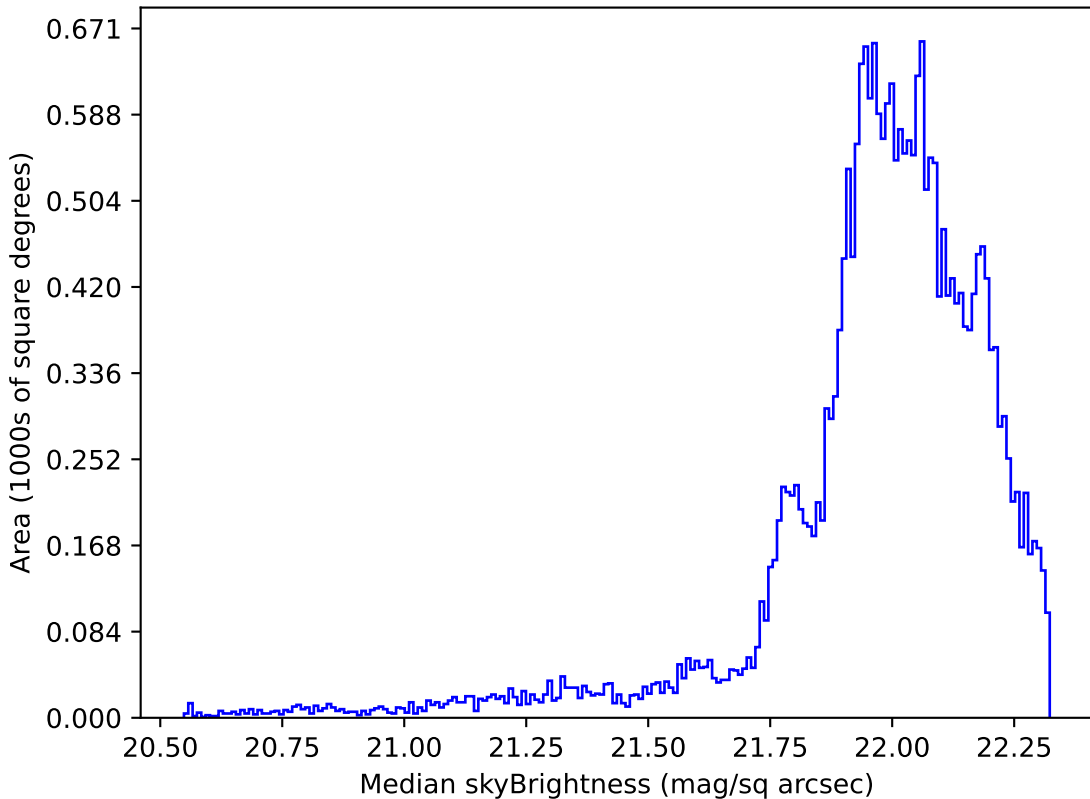
too_ignore_100_1v3.4_10yrs Yr 1 g band: Median skyBrightness
