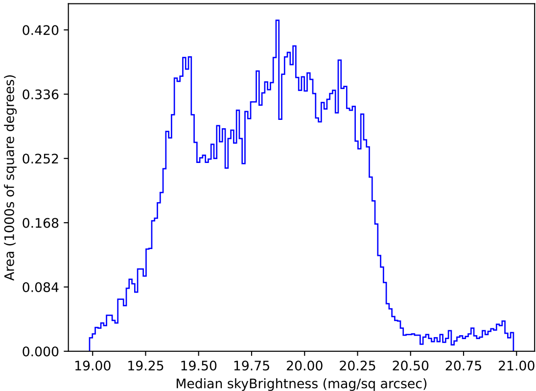
too_ignore_100_1v3.4_10yrs Yr 1 all bands: Median skyBrightness
