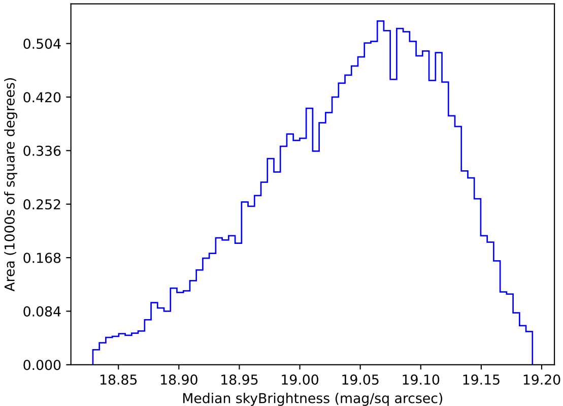
too_ignore_100_1v3.4_10yrs WFD z band: Median skyBrightness
