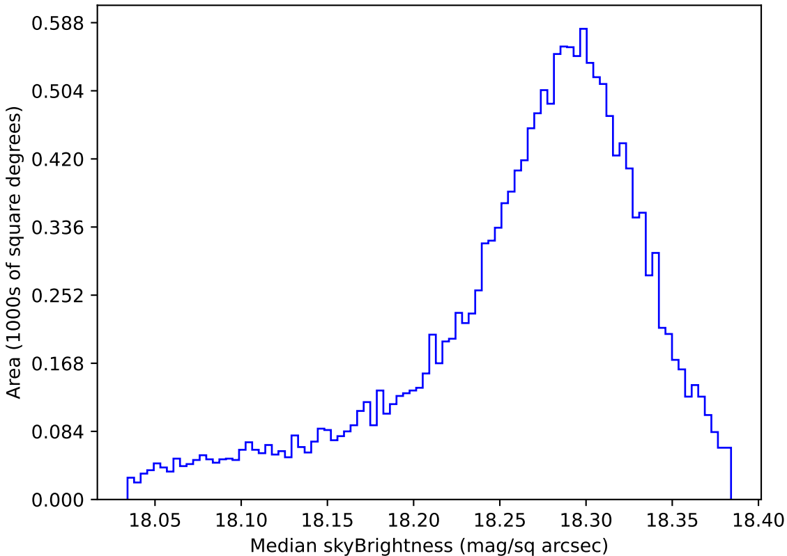
too_ignore_100_1v3.4_10yrs WFD y band: Median skyBrightness
