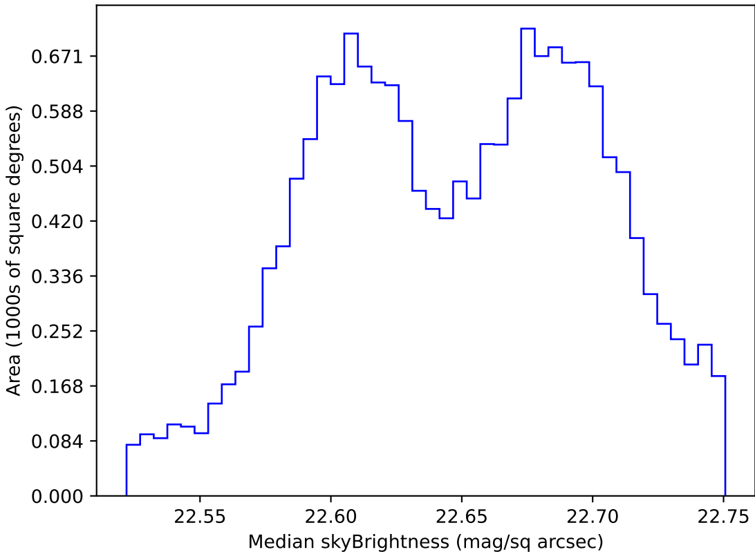
too_ignore_100_1v3.4_10yrs WFD u band: Median skyBrightness
