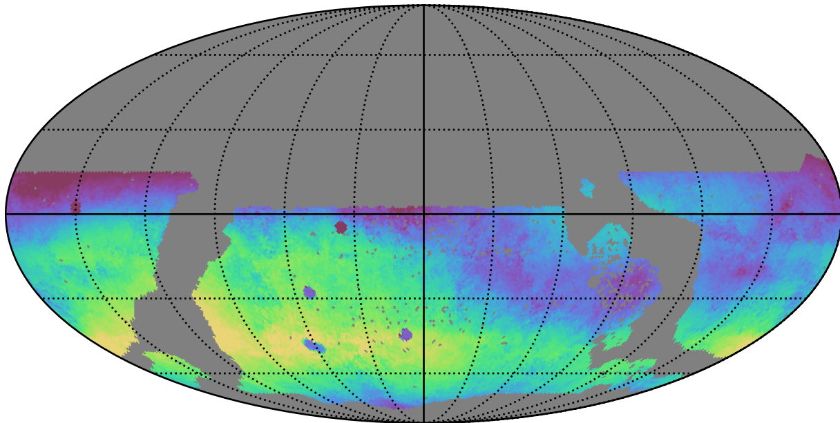
too_ignore_100_1v3.4_10yrs WFD r band: Median skyBrightness
