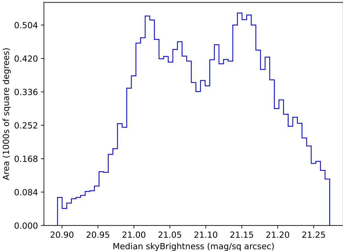
too_ignore_100_1v3.4_10yrs WFD r band: Median skyBrightness
