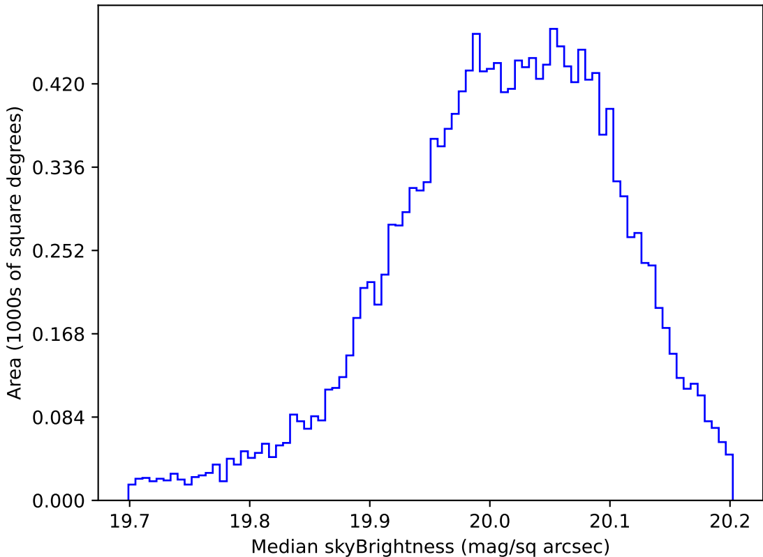
too_ignore_100_1v3.4_10yrs WFD i band: Median skyBrightness
