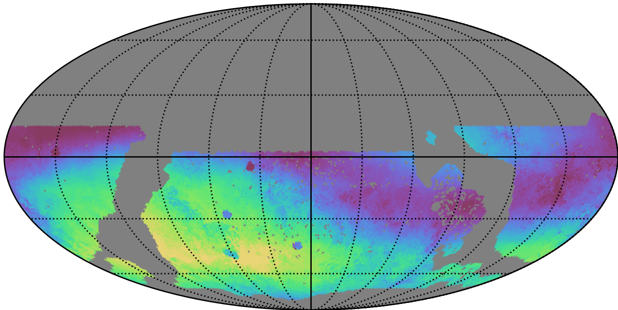
too_ignore_100_1v3.4_10yrs WFD g band: Median skyBrightness
