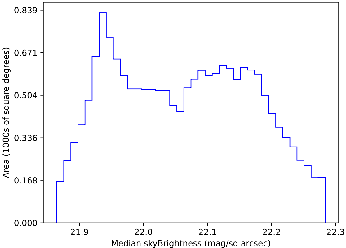
too_ignore_100_1v3.4_10yrs WFD g band: Median skyBrightness
