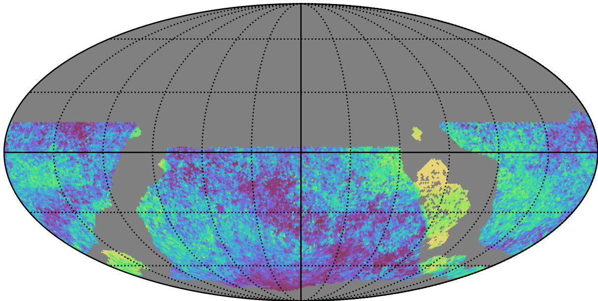
too_ignore_100_1v3.4_10yrs WFD all bands: Median skyBrightness
