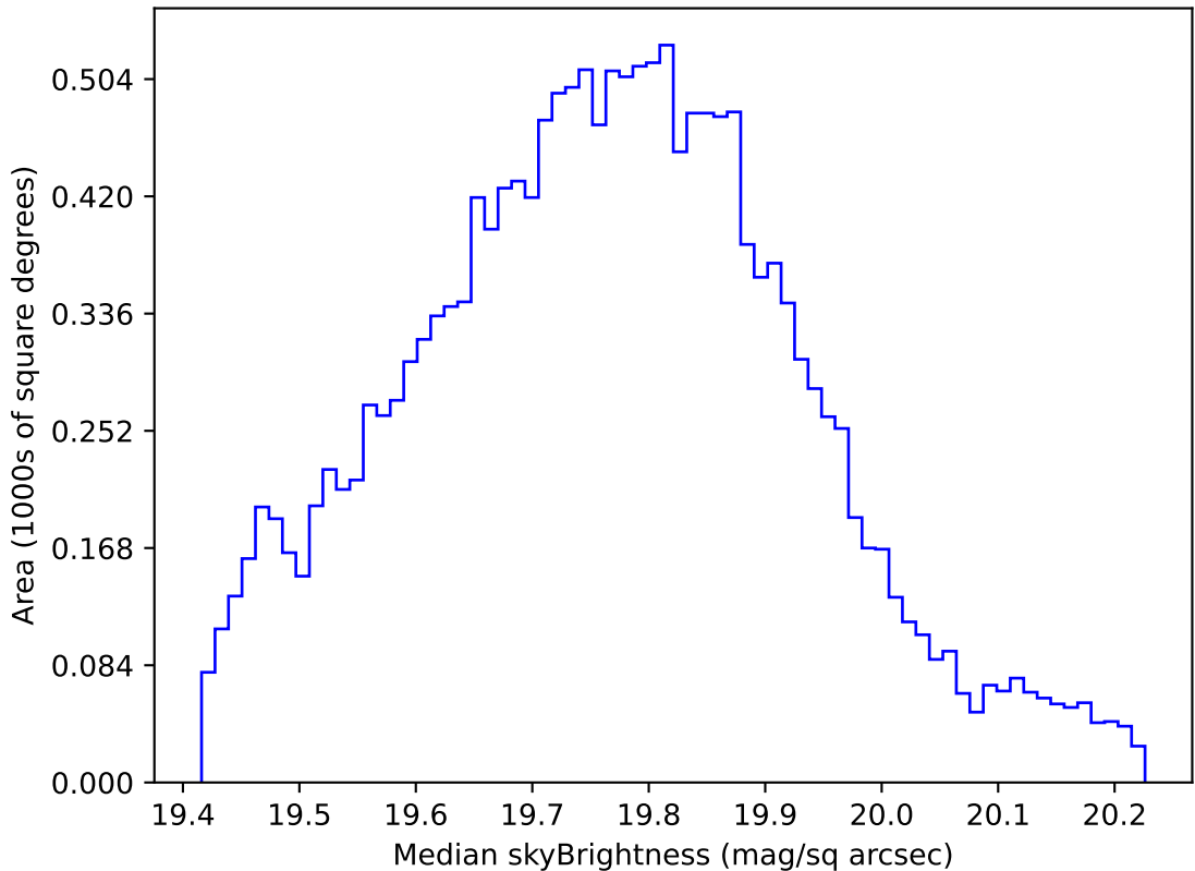
too_ignore_100_1v3.4_10yrs WFD all bands: Median skyBrightness
