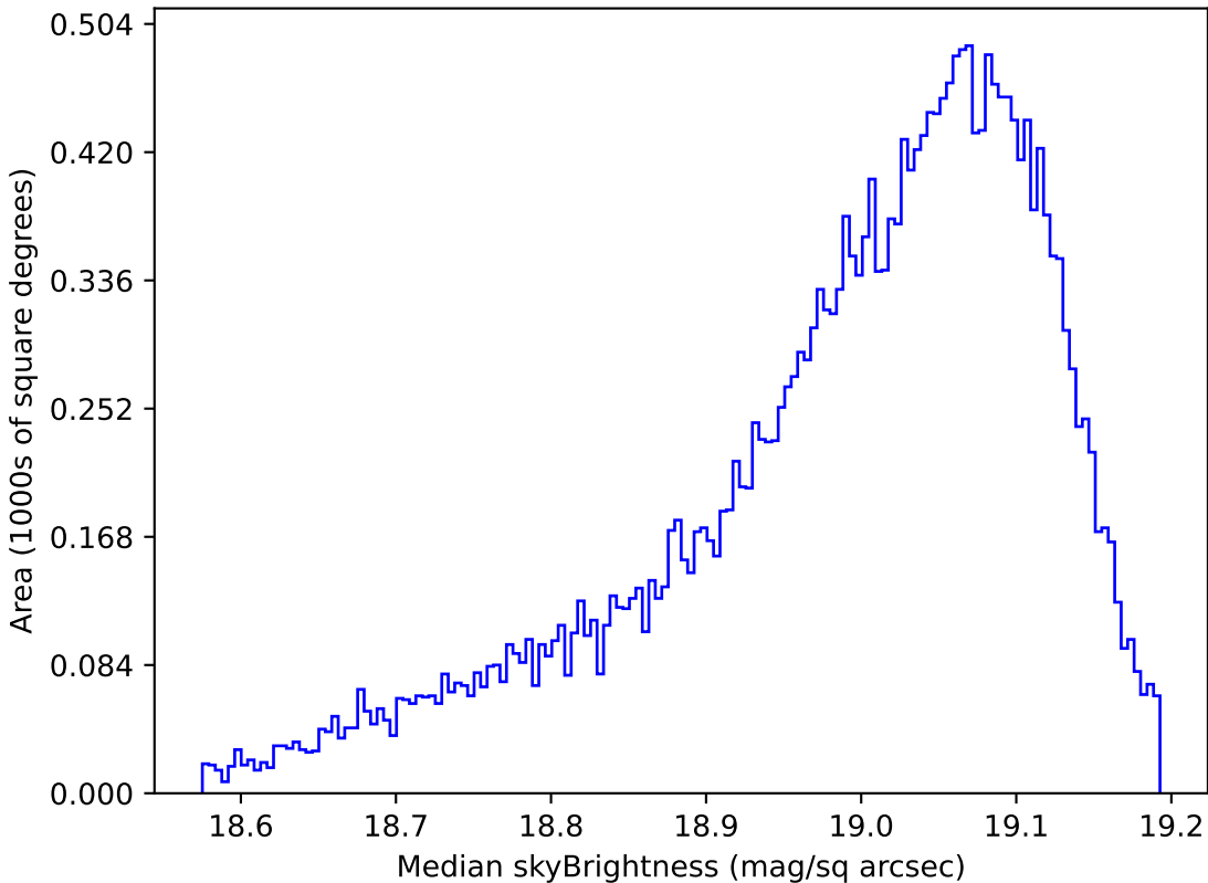
too_ignore_100_1v3.4_10yrs All sky z band: Median skyBrightness
