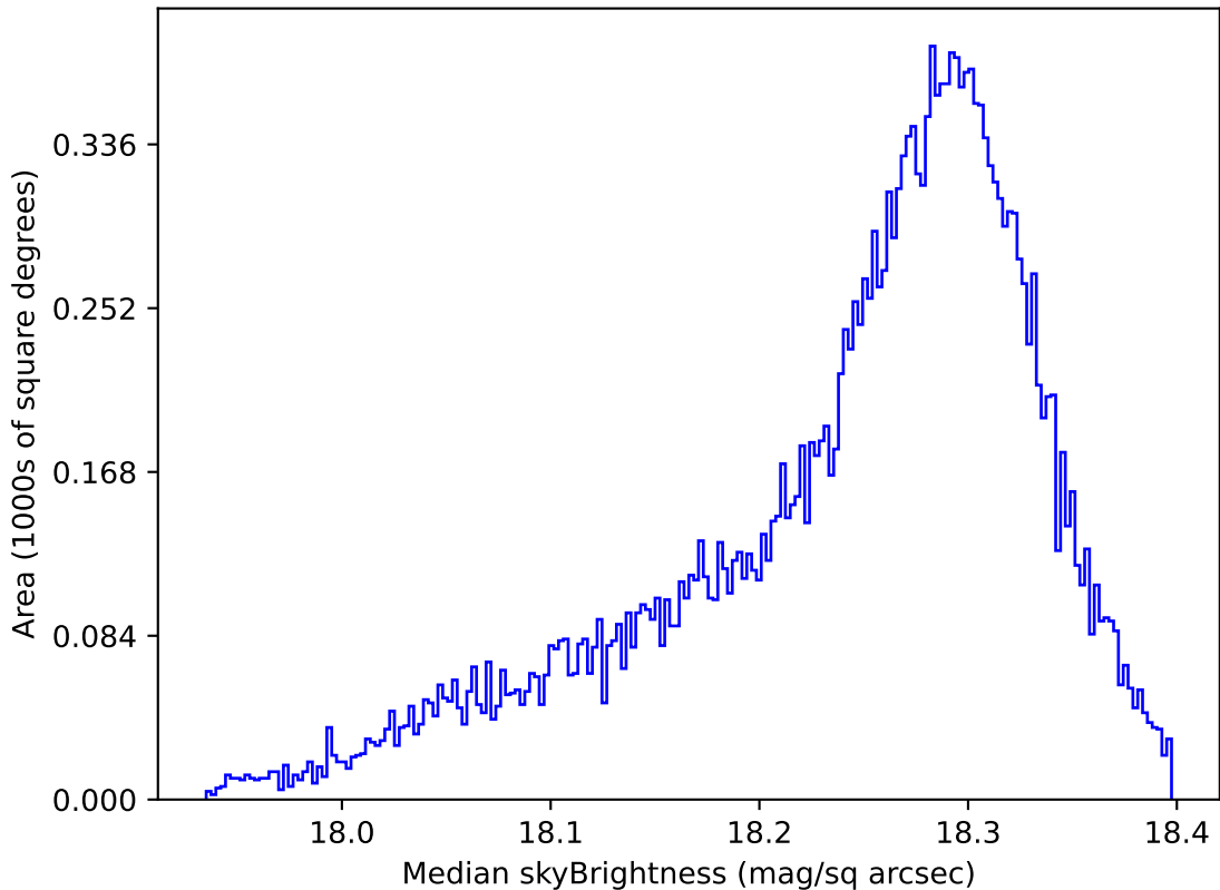
too_ignore_100_1v3.4_10yrs All sky y band: Median skyBrightness
