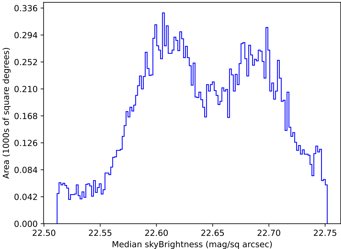
too_ignore_100_1v3.4_10yrs All sky u band: Median skyBrightness
