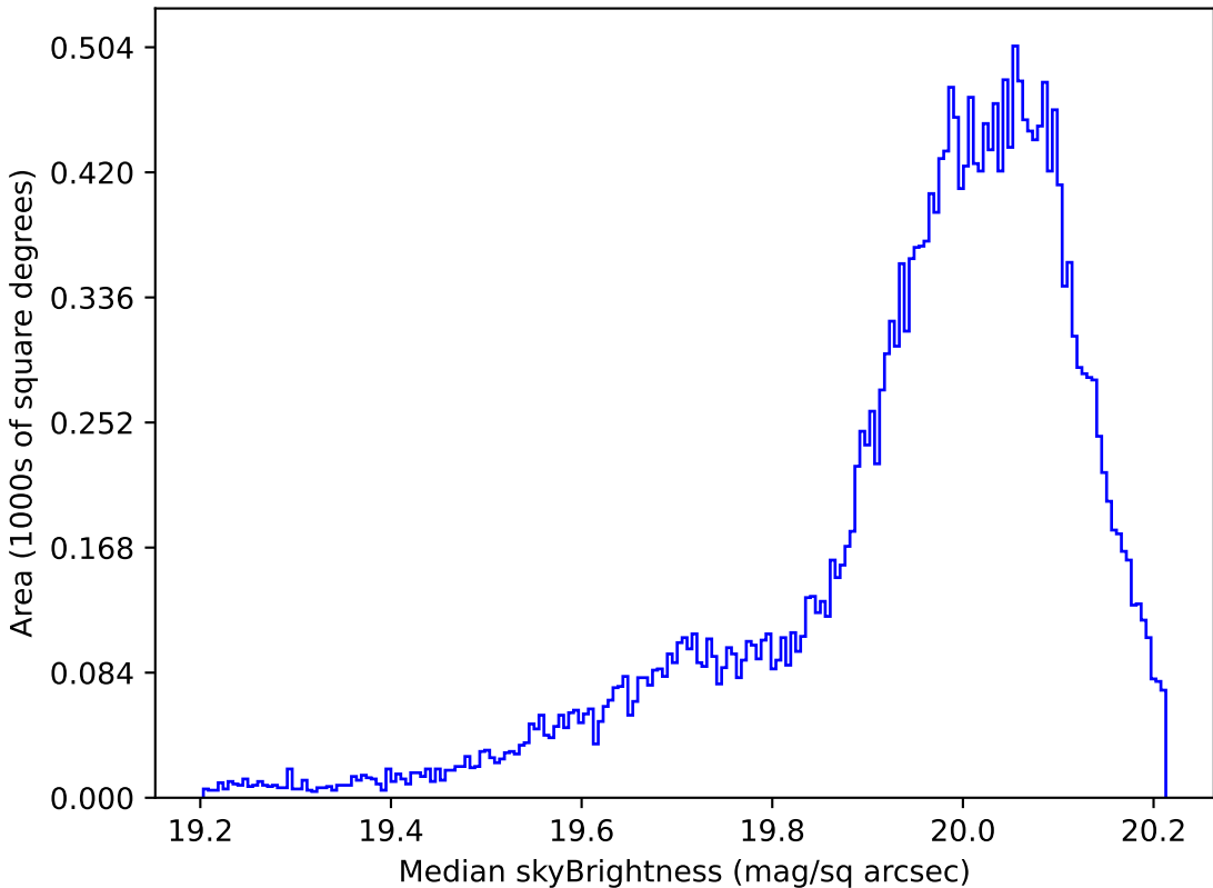
too_ignore_100_1v3.4_10yrs All sky i band: Median skyBrightness
