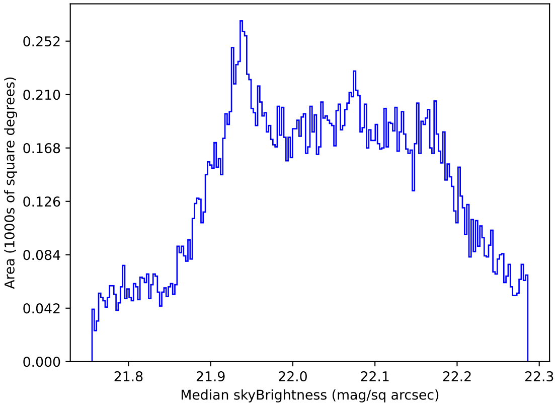
too_ignore_100_1v3.4_10yrs All sky g band: Median skyBrightness
