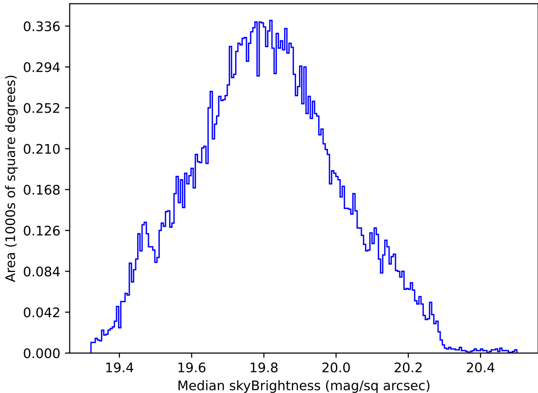
too_ignore_100_1v3.4_10yrs All sky all bands: Median skyBrightness
