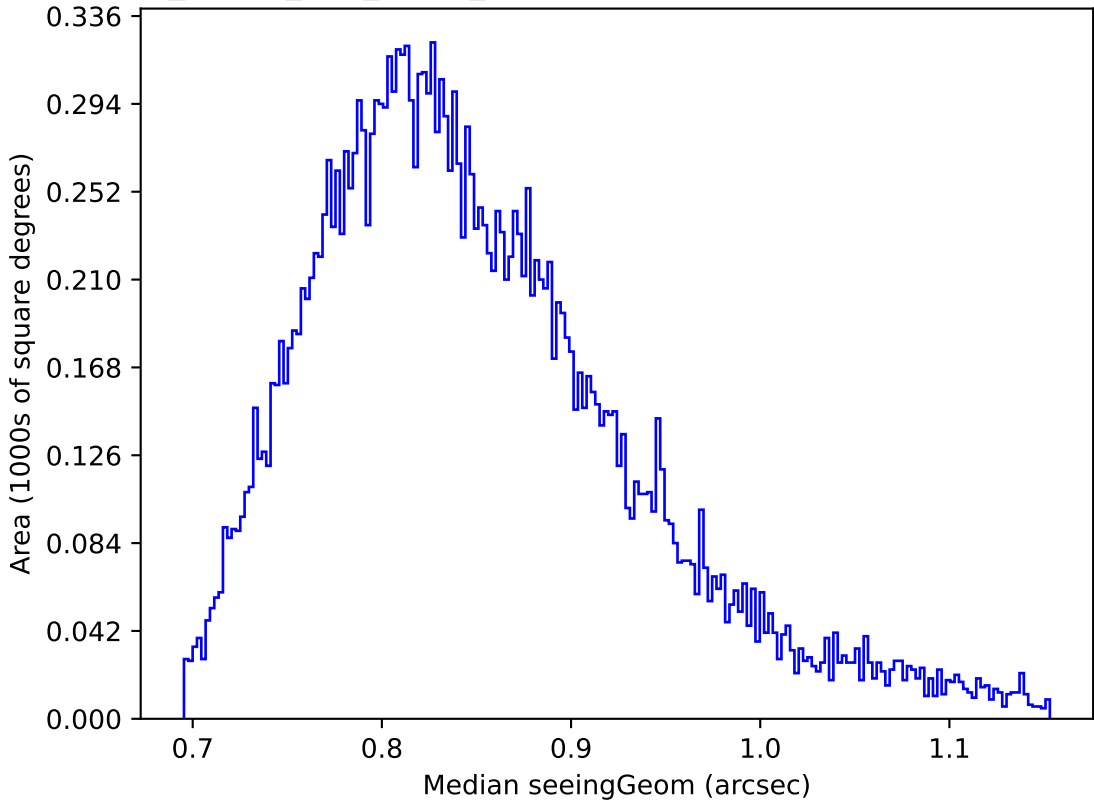
too_ignore_100_1v3.4_10yrs Yr 1 y band: Median seeingGeom
