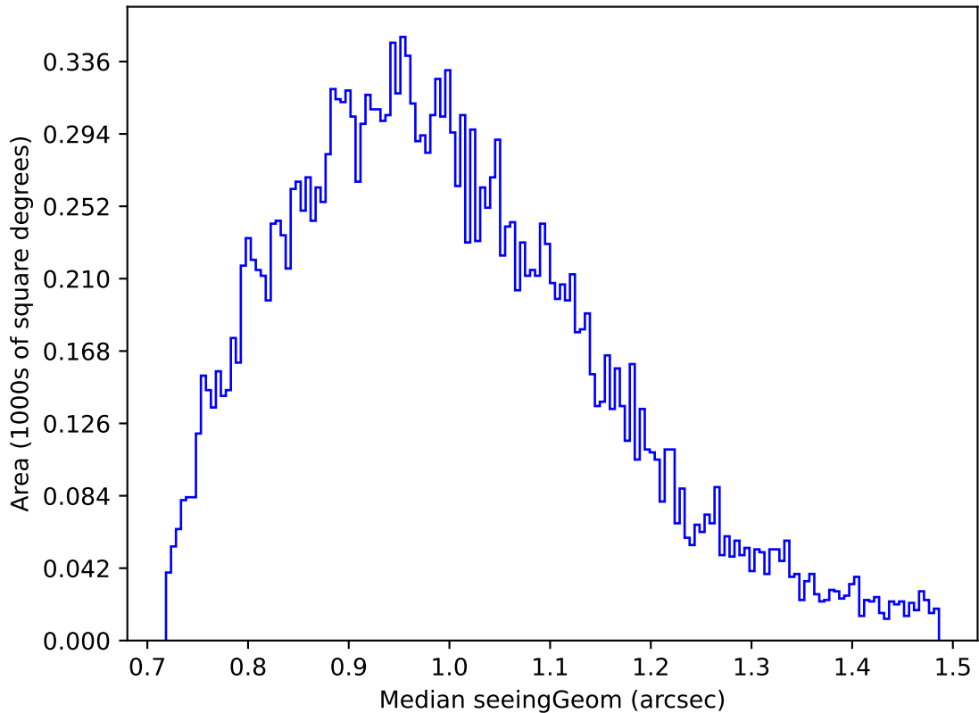
too_ignore_100_1v3.4_10yrs Yr 1 u band: Median seeingGeom
