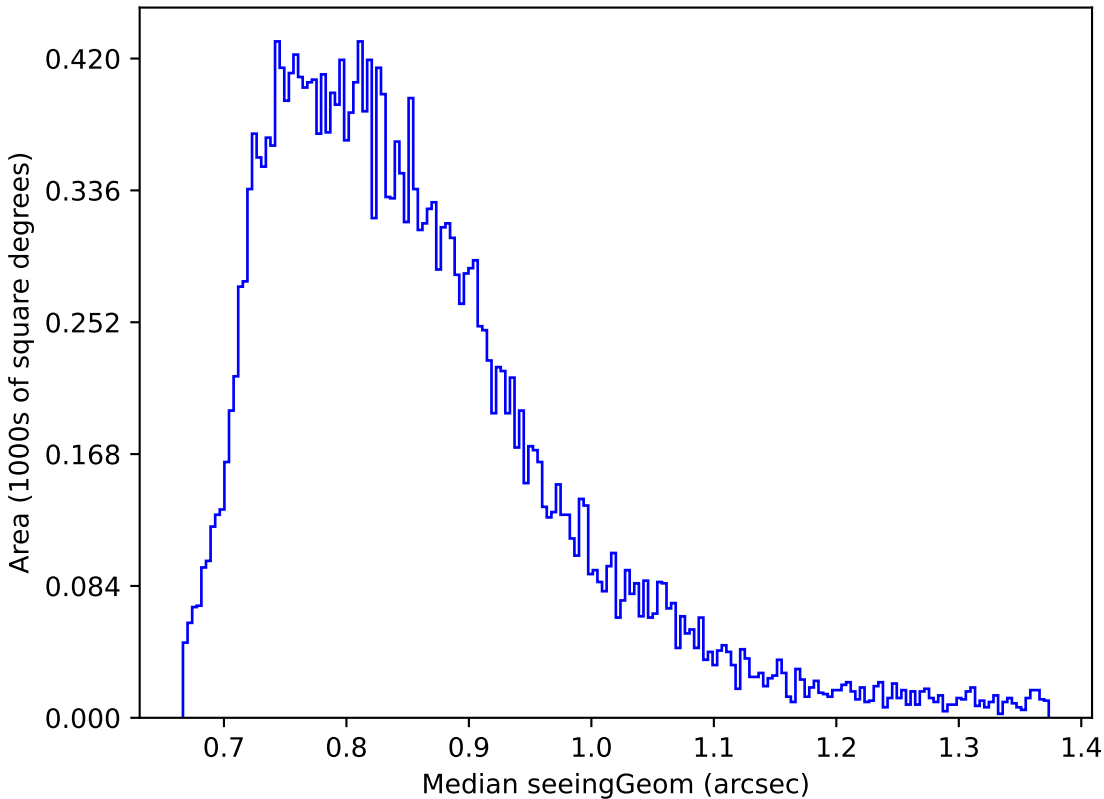
too_ignore_100_1v3.4_10yrs Yr 1 r band: Median seeingGeom
