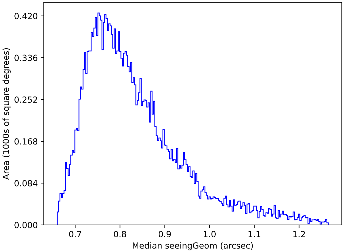
too_ignore_100_1v3.4_10yrs Yr 1 i band: Median seeingGeom
