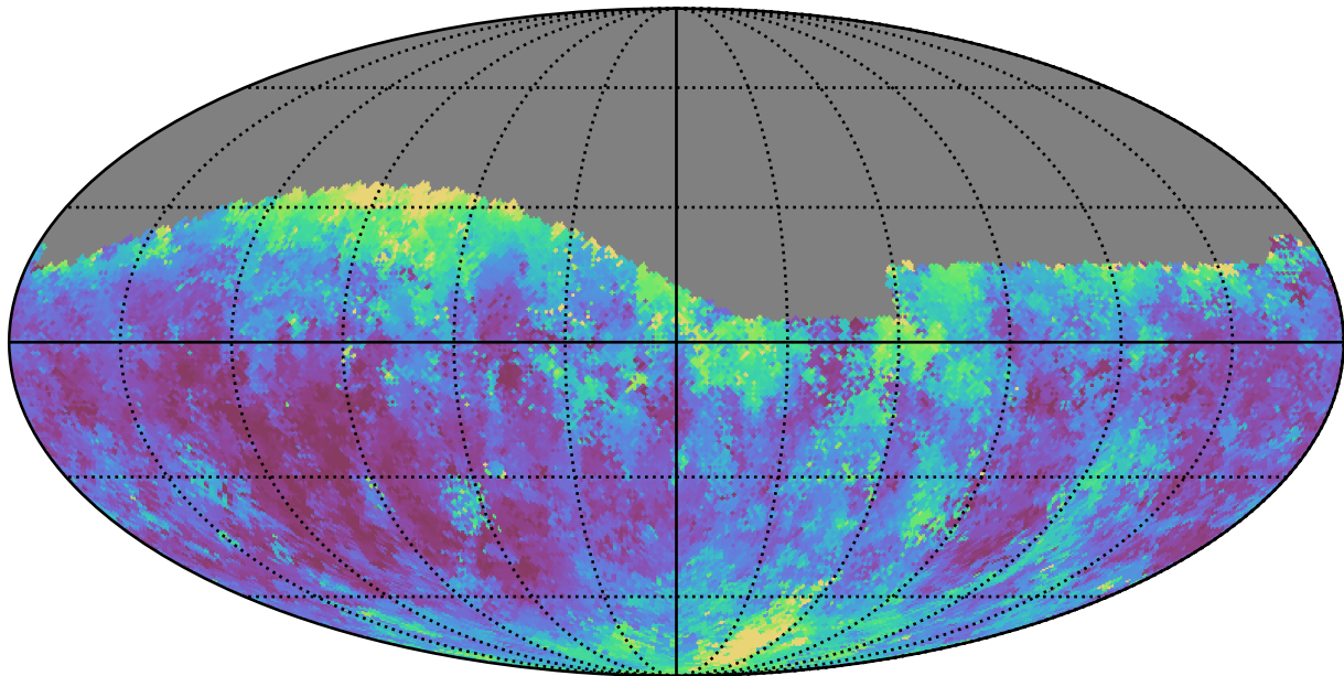
too_ignore_100_1v3.4_10yrs Yr 1 g band: Median seeingGeom
